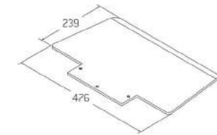
Toe plate GS-NG [476x239x7 mm] for goods in cartons [e.g. beverage cans] Art. no. 930 084
